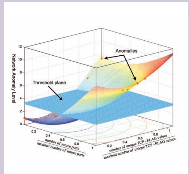
Figure 3●Sensing the port scan by detecting anomaly values
