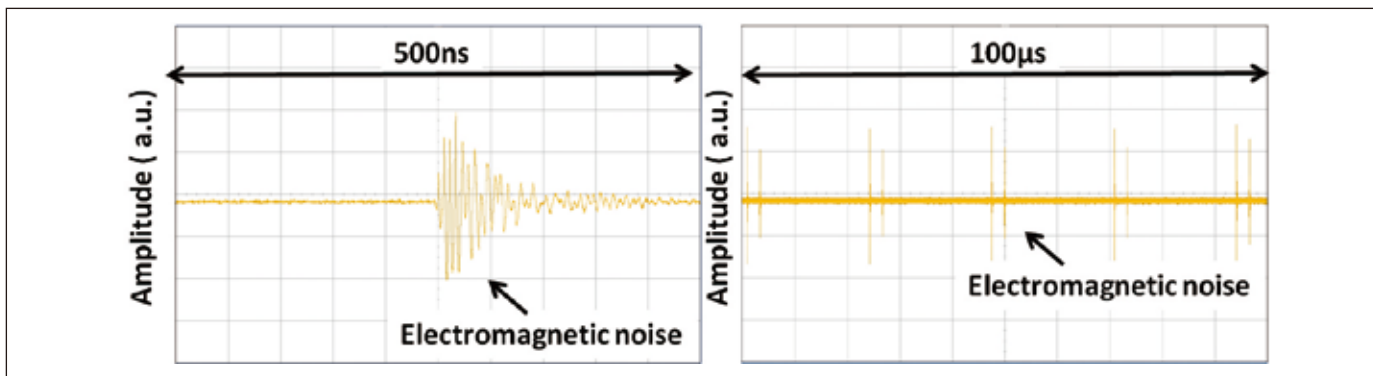
Figure 2 ● Radiation noise waveform from LED lamp
