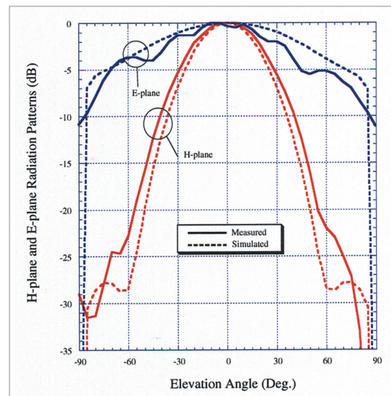
Fig.8 Simulated and measured patterns of CPA (at 10GHz)
