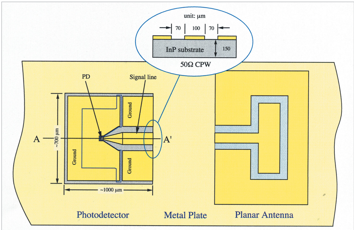
Fig. 4 Configuration of a photodetector and a planar antenna to be integrated with the PD
