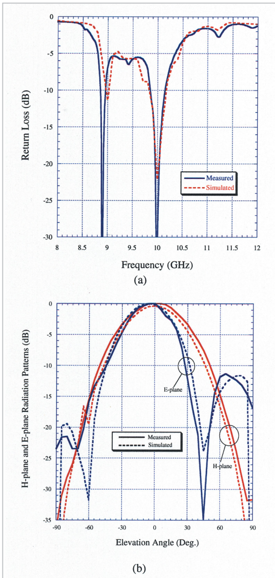
Fig.9 Simulated and measured return loss and patterns of CPA array (at 10GHz)
