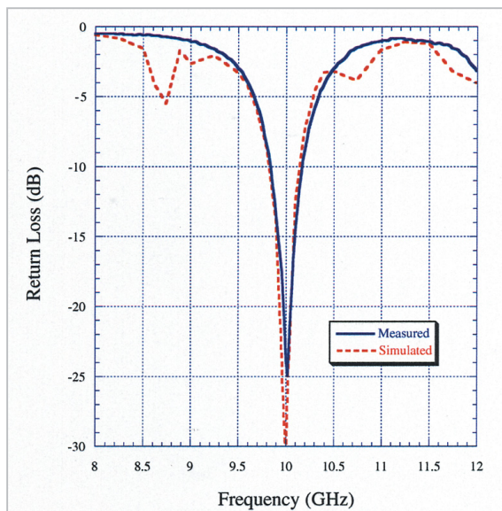
Fig.7 Simulated and measured return loss of CPA (at 10GHz)
