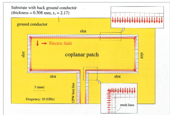
Fig. 6 Electric field distribution along the slots in CPA
