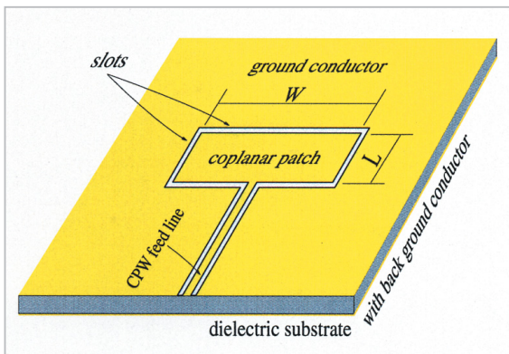
Fig. 5 Coplanar patch antenna (CPA) with a coplanar feeding structure
