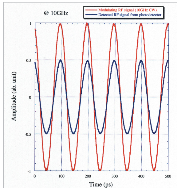
Fig.11 Waveform of the modulating signal (CW) and output signal from the PD
