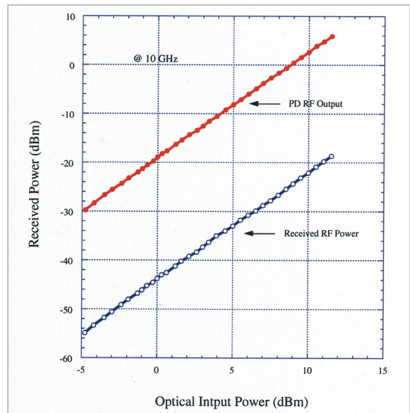
Fig.10 RF power generated by PD and received by horn antenna
