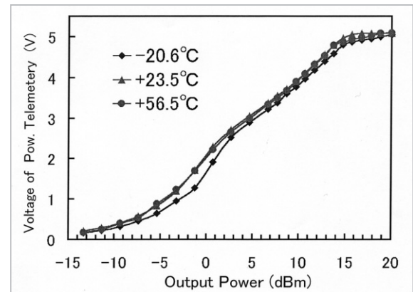
Fig.4 Telemetry voltage versus output power
