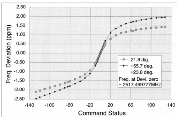
Fig.7 Local signal frequency deviation versus command status
