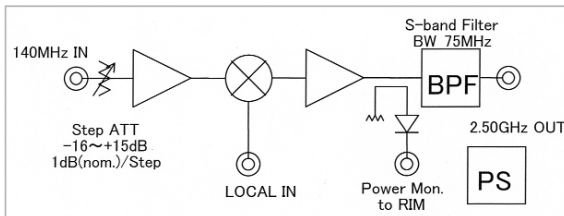
Fig.2 Block diagram of transmission-frequency converter
