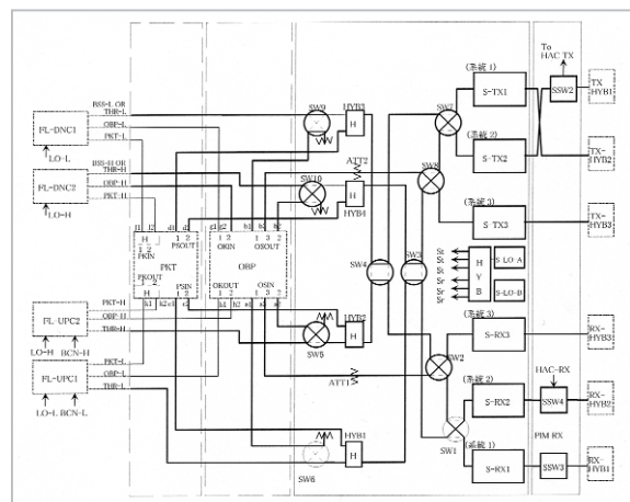
Fig. 1 Block diagram of S-band converter
