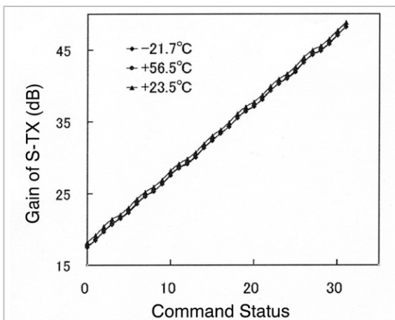
Fig.3 Characteristics of gain-adjustment function
