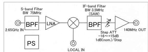
Fig.5 Block diagram of received-frequency converter
