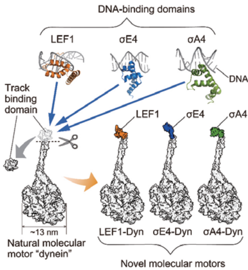
Figure 2 Conceptual diagram illustrating how a new molecular machine can be created by fusing a DNA-binding protein to dynein, a naturally occurring molecular motor
