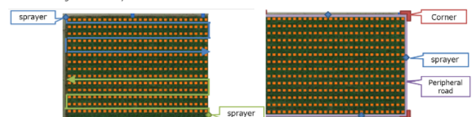
Fig.5 : Emulation of sprayers movement in orchard
