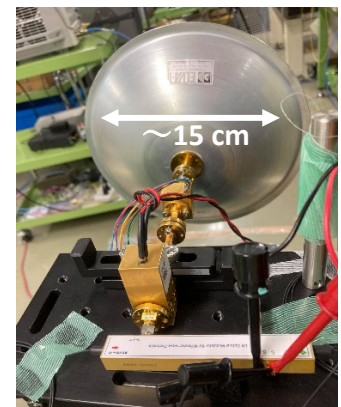
Fig.5 : Proof-of-concept demonstration system for photonic downconversion
