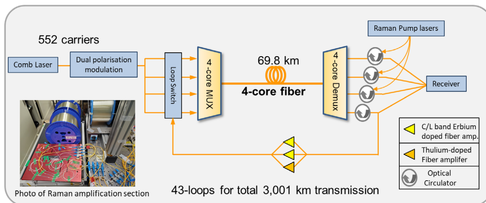
Fig.4 : Schematic diagram of the 4-core optical fiber transmission system
