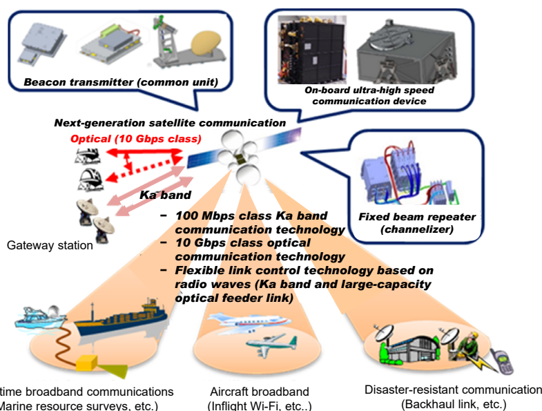
Fig. 7 : Flexible link technologies onboard ETS-9
