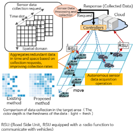
Fig.2 : Sensor network for drive automation
