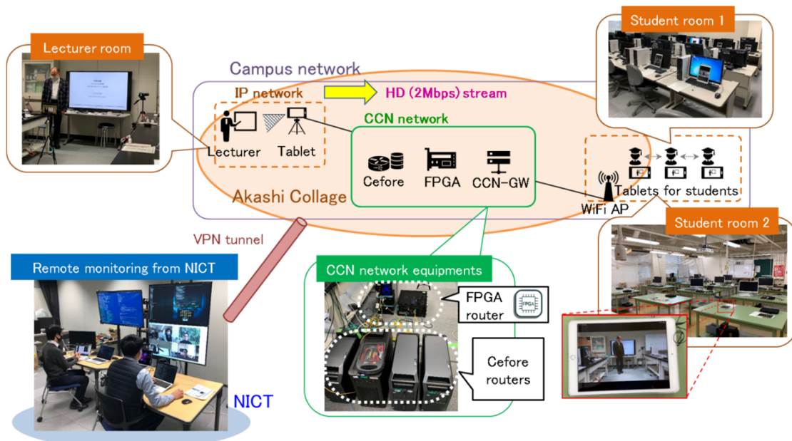
Fig.3 : Outline of systems in remote classroom
