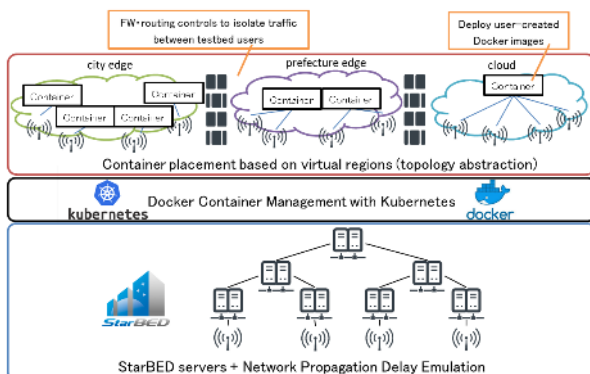
Fig.3 : Edge computing testbed
