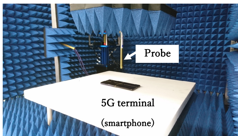
Fig.5 : Measurement system for a compliance test of a 5G terminal to RF safety guidelines.
