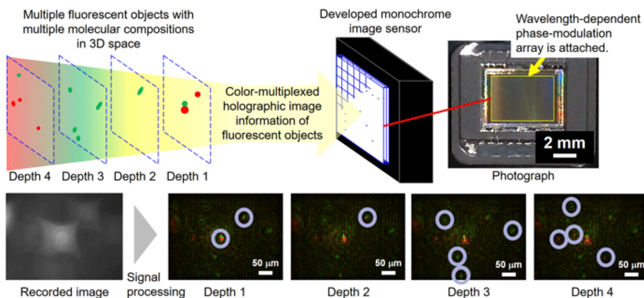
Fig.7 : Holographic microscope
