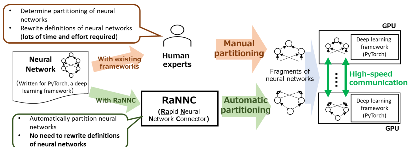
Fig. : Parallel training of large-scale neural networks
