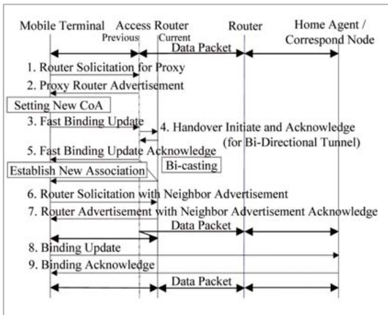
Fig.7 Mobile IPv6 Fast Handoff Procedure
