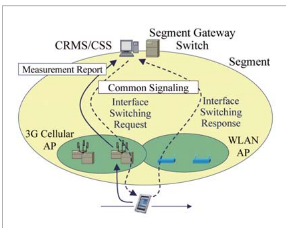
Fig.5 Fast Vertical Handover
