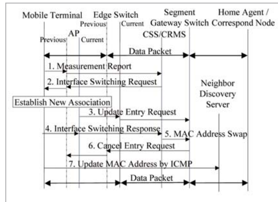
Fig.8 Fast Vertical Handover Procedure
