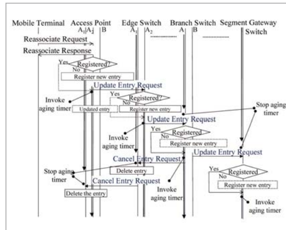
Fig.3 Update and Cancel Entry on Intra-Segment
