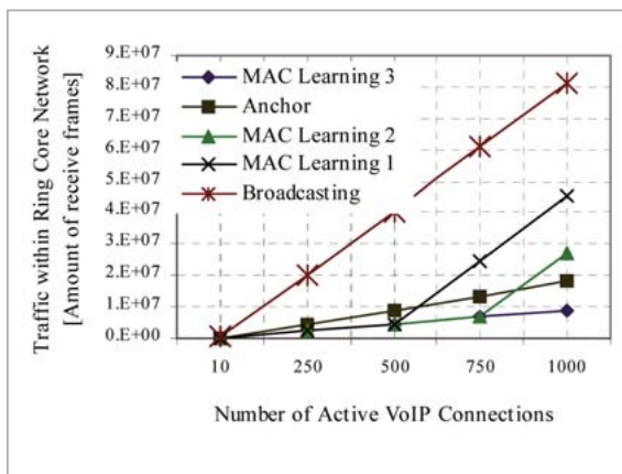
Fig.6 Evaluation of the Inter-Segment Ring Mobility
